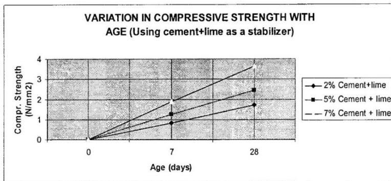
Figure 7: Variation in Compressive Strength with Age with cement and lime as a binder
