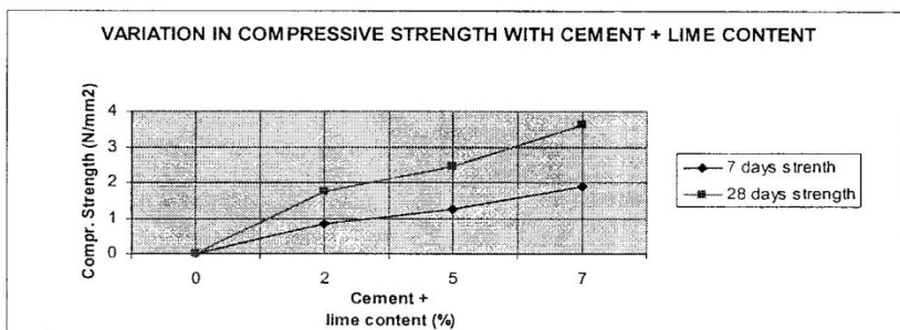
Figure 5: Variation in strength with cement plus lime content
