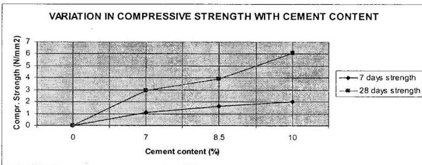
Figure 4: Variation in strength with cement content
