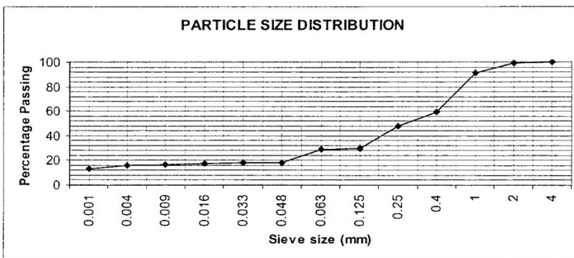
Figure 3: Particle Size Distribution
