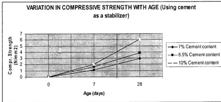
Figure 6: Variation in Compressive Strength with Age with cement as a binder
