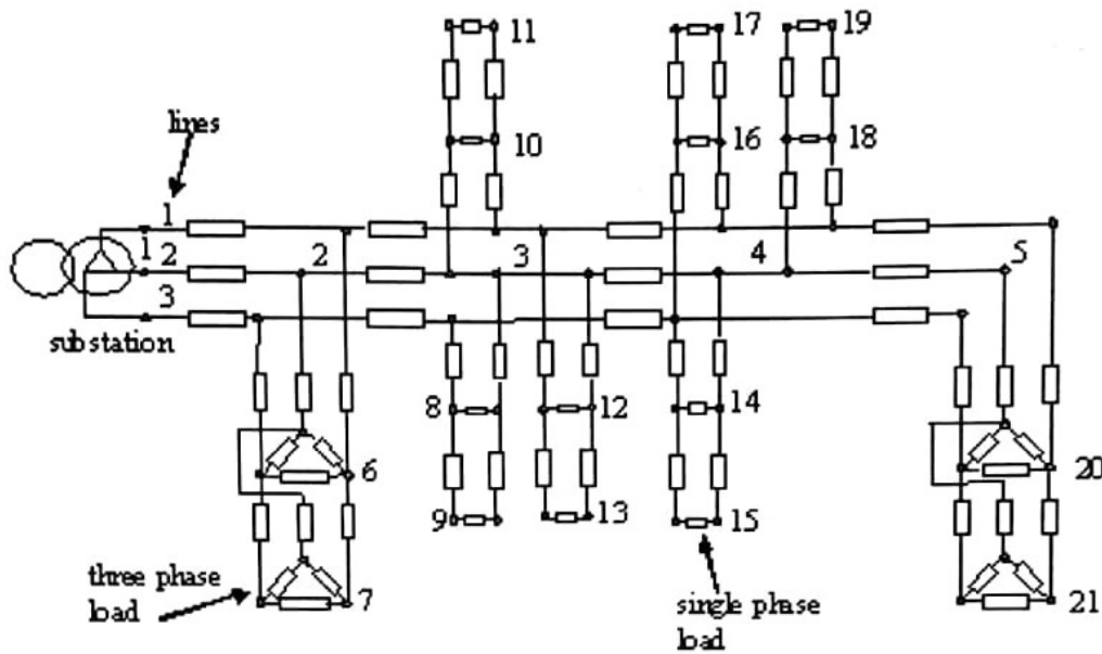
Figure A1: Three-phase backbone feeder tapped by single-phase, SWER and three-phase topologies used to test the proposed method.
